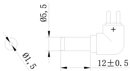
1. DETACHABLE PLUG. BLACK PLASTIC RING HARDWARE. Ø1.50x5.50x12.0±0.5mm, "L"TYPE. USED 30P BLACK COLOR PVC.
