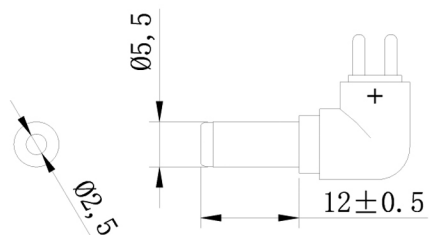
2. DETACHABLE PLUG. RED PLASTIC RING HARDWARE. Ø2.50x5.50x12.0±0.5mm, "L"TYPE. USED 30P BLACK COLOR PVC.
