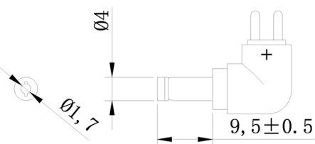
4. DETACHABLE PLUG. YELLOW PLASTIC RING HARDWARE. Ø1.70x4.00x9.5±0.5mm, "L"TYPE. USED 30P BLACK COLOR PVC.
