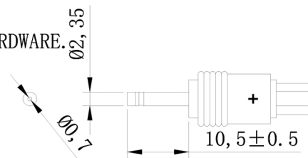
7. DETACHABLE PLUG. YELLOW PLASTIC RING HARDWARE. Ø0.70x2.35x10.5±0.5mm, "I"TYPE. USED 30P BLACK COLOR PVC.
