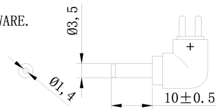
6. DETACHABLE PLUG. BLUE PLASTIC RING HARDWARE. Ø1.40x3.50x10.0±0.5mm, "L"TYPE. USED 30P BLACK COLOR PVC.
