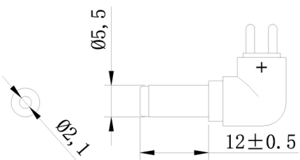
3. DETACHABLE PLUG. ORANGE PLASTIC RING HARDWARE. Ø2.10x5.50x12.0±0.5mm, "L"TYPE. USED 30P BLACK COLOR PVC.
