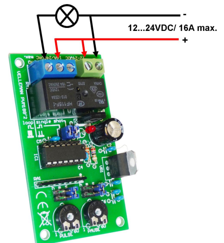
CONNECTION EXEMPLE: LOW VOLTAGE
