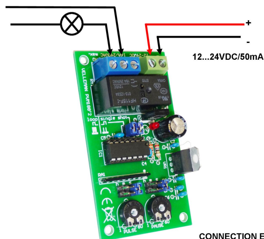
CONNECTION EXEMPLE: LOW VOLTAGE
